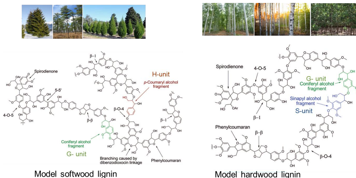
Figure 1.4. Native lignin structure (adopted from Zakzeski et al., 2010 and Ralph et al., 2004).
