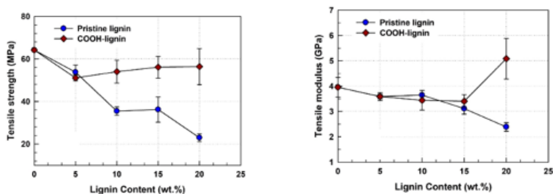
Figure 2.16. Tensile strength and tensile modulus of PLA composites with modified and unmodified lignin (Hong et al., 2021).
