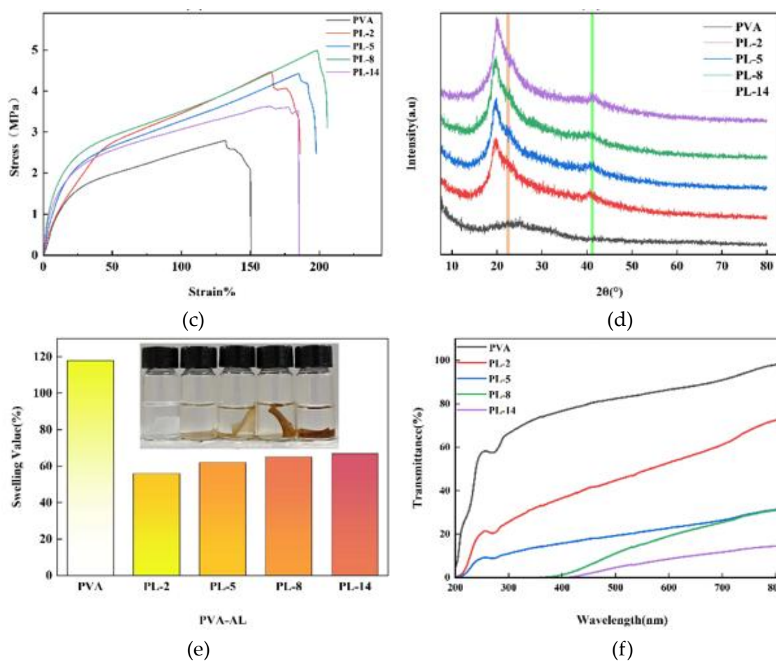
Figure 2.13. Infrared spectra (a), thermogravimetric (b), stress–strain (c), XRD (d), solubility (e), and UV optical resistance (f) of PVA, PL-2, PL-5, PL-8, and PL-14 (Liu et al., 2024).
